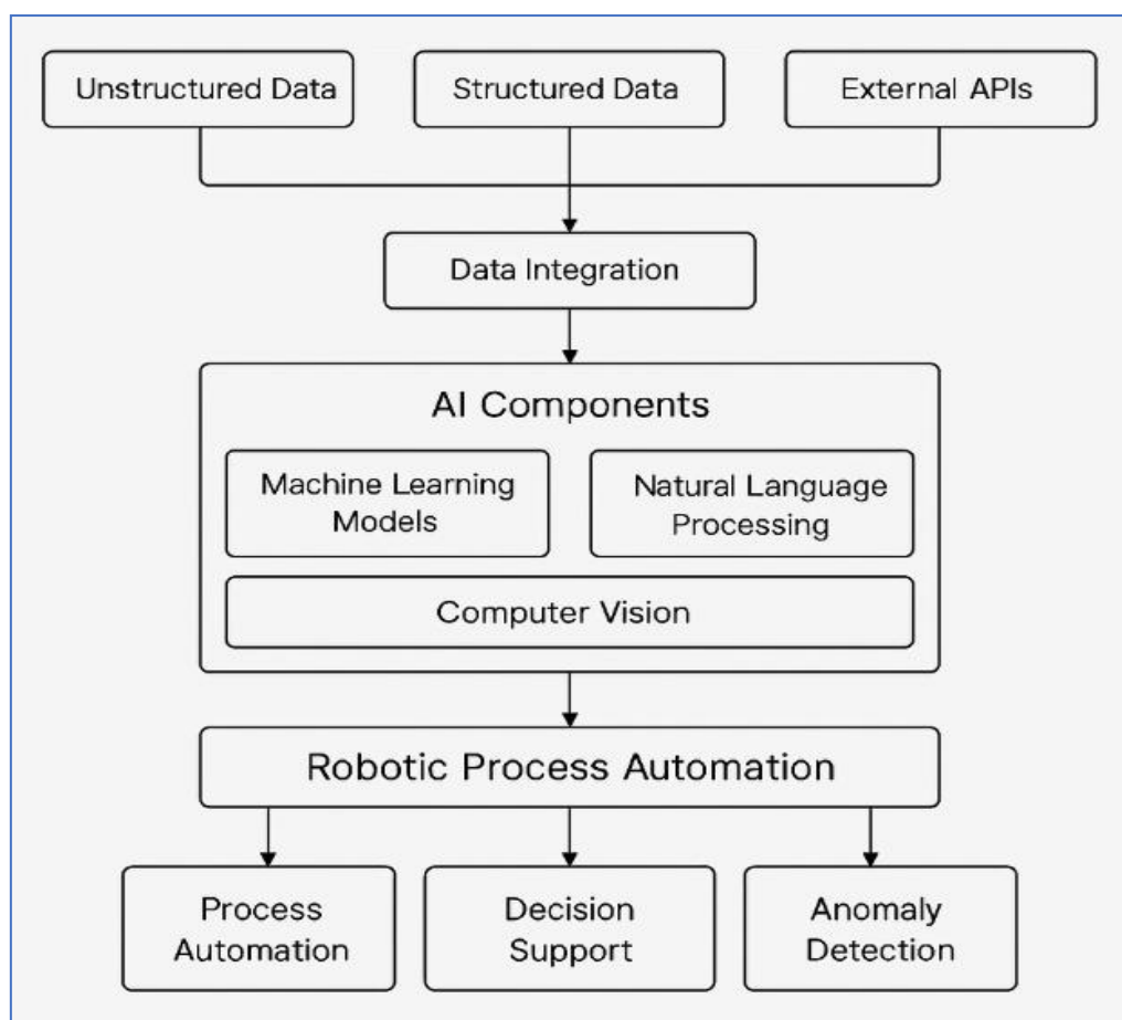
Fig. 1. Reference Architecture of AI-Augmented IPA System
